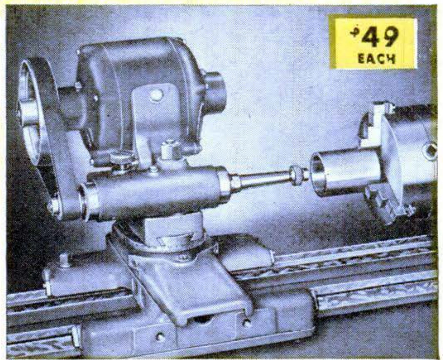
Internal Grinding Attachment
